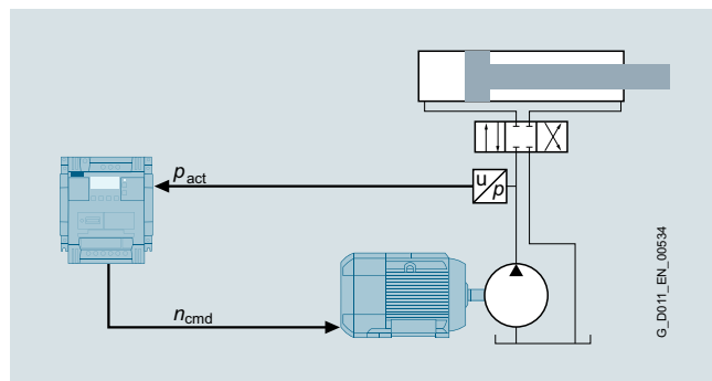
Example of block diagram for a variable-speed pump with SINAMICS V20
