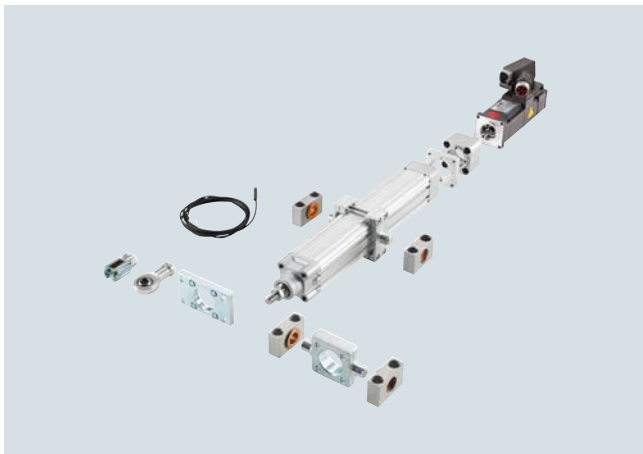
Axial mounting of a SIMOTICS S-1FK7 motor on the linear unit with mounting kit and accessories
