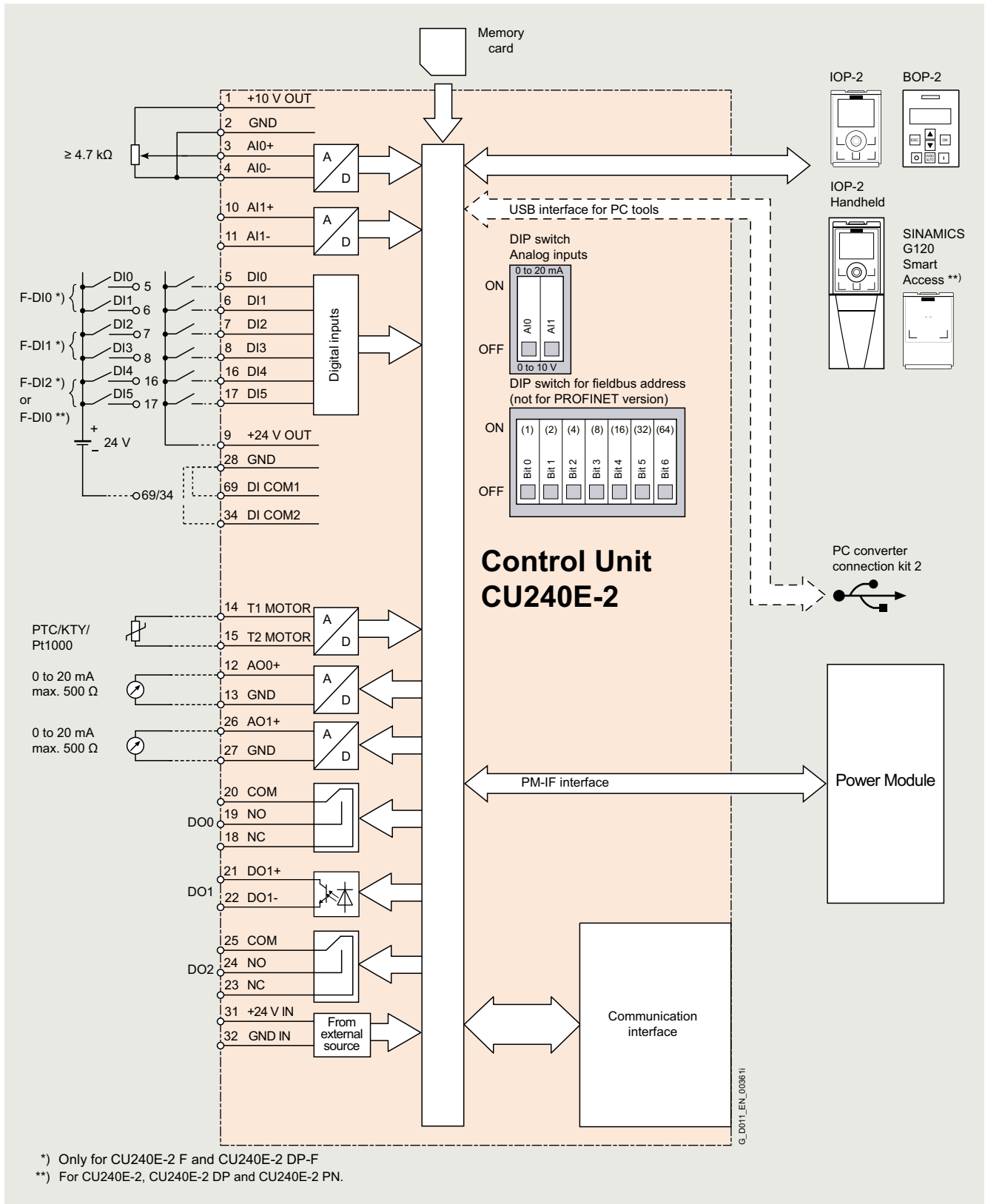
Connection example of a CU240E-2 series Control Unit
