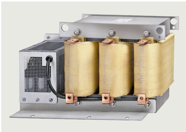
Sine-wave filter
