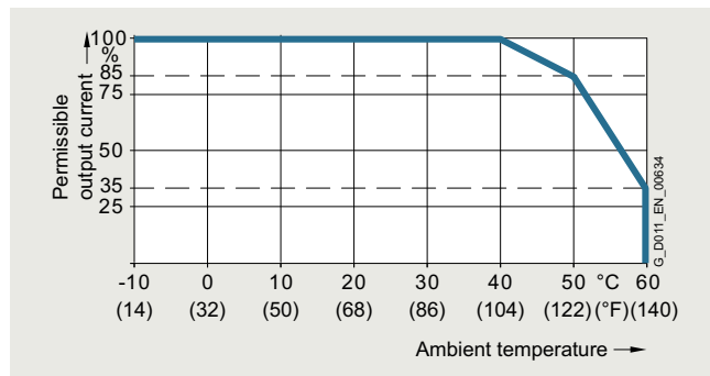
Permissible output current as a function of ambient temperature for low overload (LO) for PM240-2 Power Modules FSA to FSC at 200 V and 400 V FSD to FSF at 690 V FSG at 400 V
