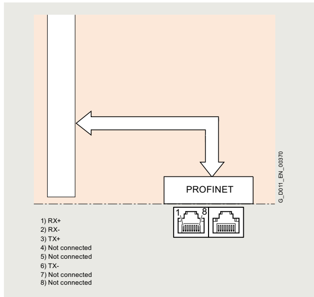
PROFINET, EtherNet/IP communication interface
