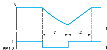
KM1: output contactor t1: deceleration without ramp (freewheel) t2: acceleration with ramp N: motor speed
