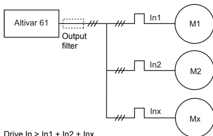
Drive I_n > I_{n1} + I_{n2} + I_{nx} Motors connected in parallel
