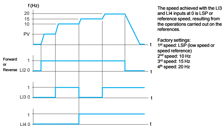
Example of operation with 4 preset speeds and 2 logic inputs
