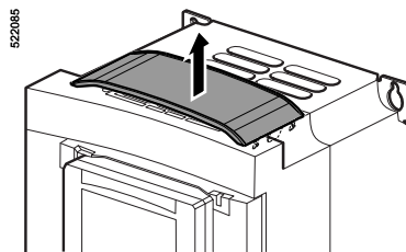
Removing the protective blanking cover from: ATV 61H●●●M3, ATV 61HD11M3X, HD15M3X, ATV 61H075N4...HD18N4
