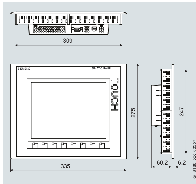
KTP1000 Basic
